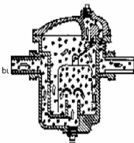
Normal steam trap operation (inverted bucket)
