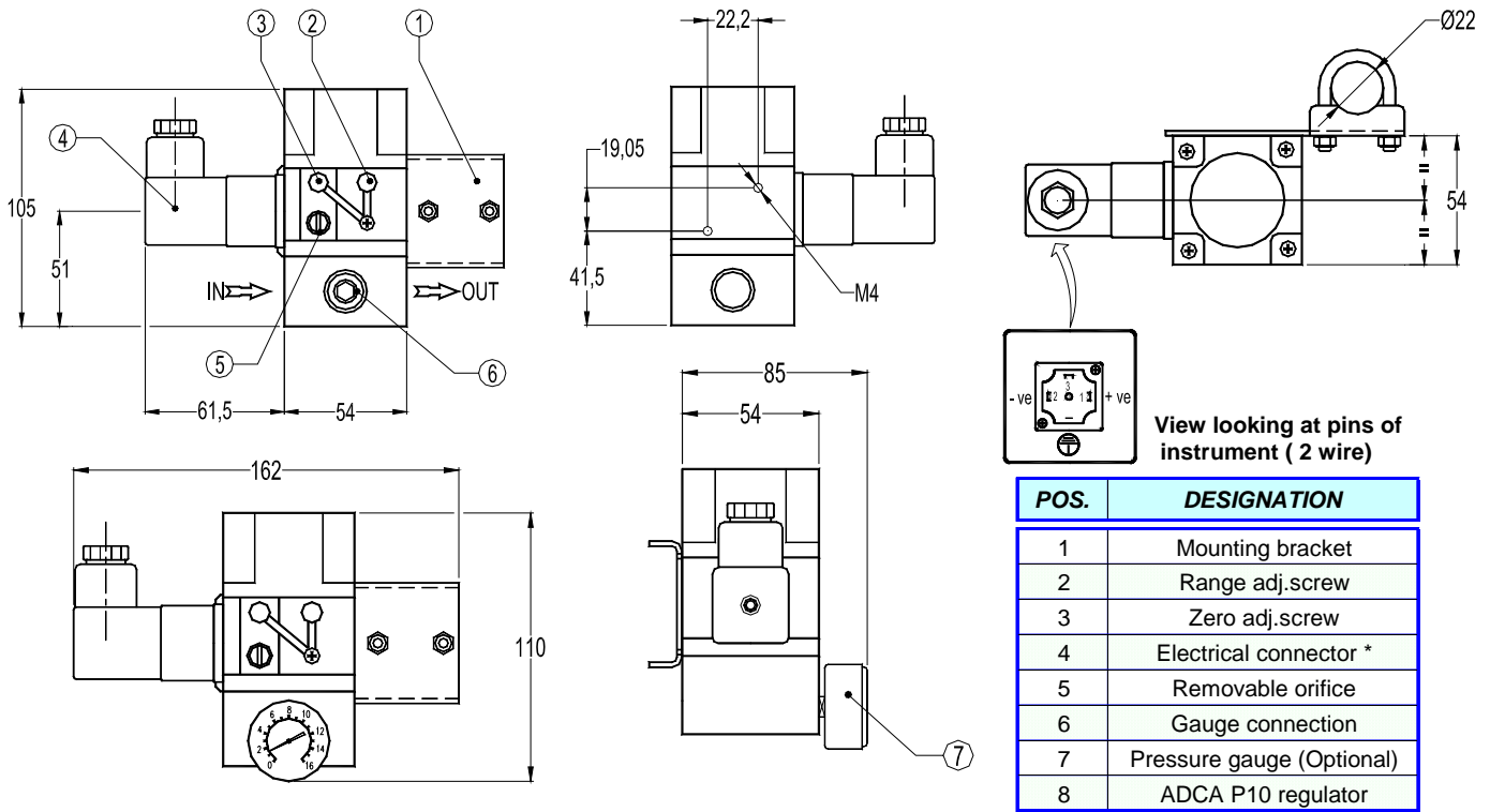
Assembling with pressure gauge (on request).
