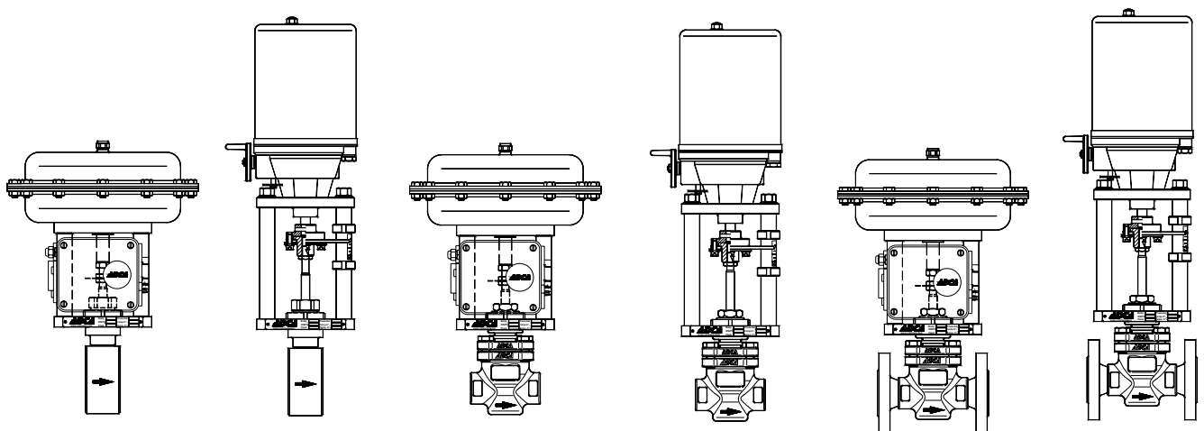
PWV / EWV Wafer type
