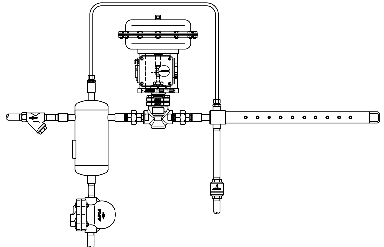
Single tube design
